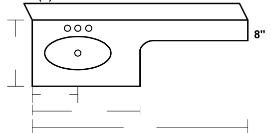
(F) BANJO STYLE OFFSET R.H SIDE
